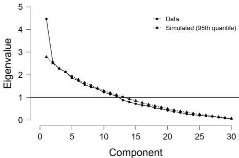
Figura 1. Scree plot
