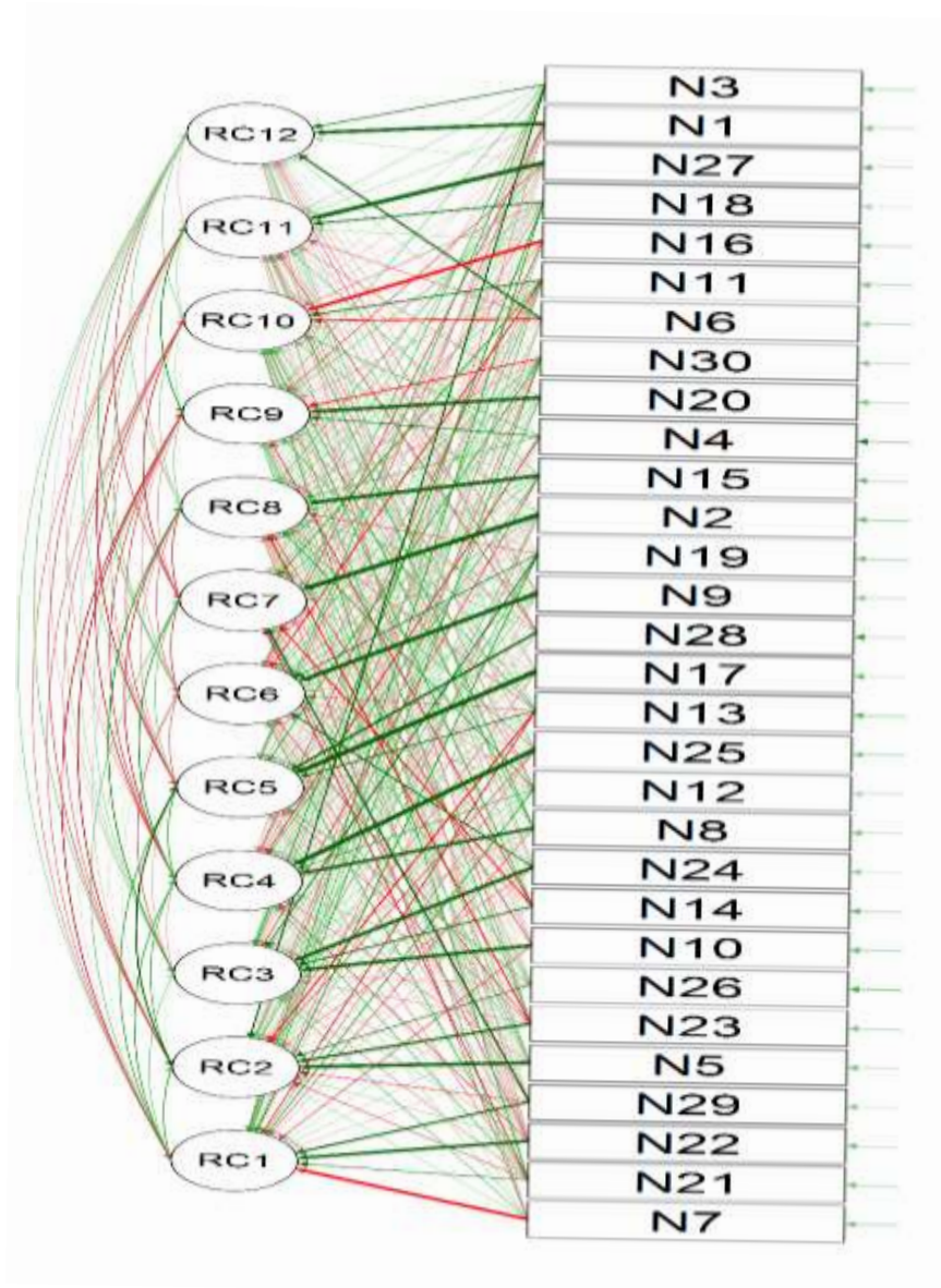
Figure 2. Path diagram
