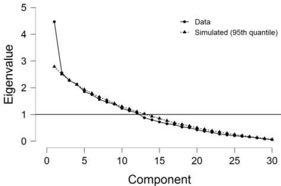
Figura 1. Scree plot
